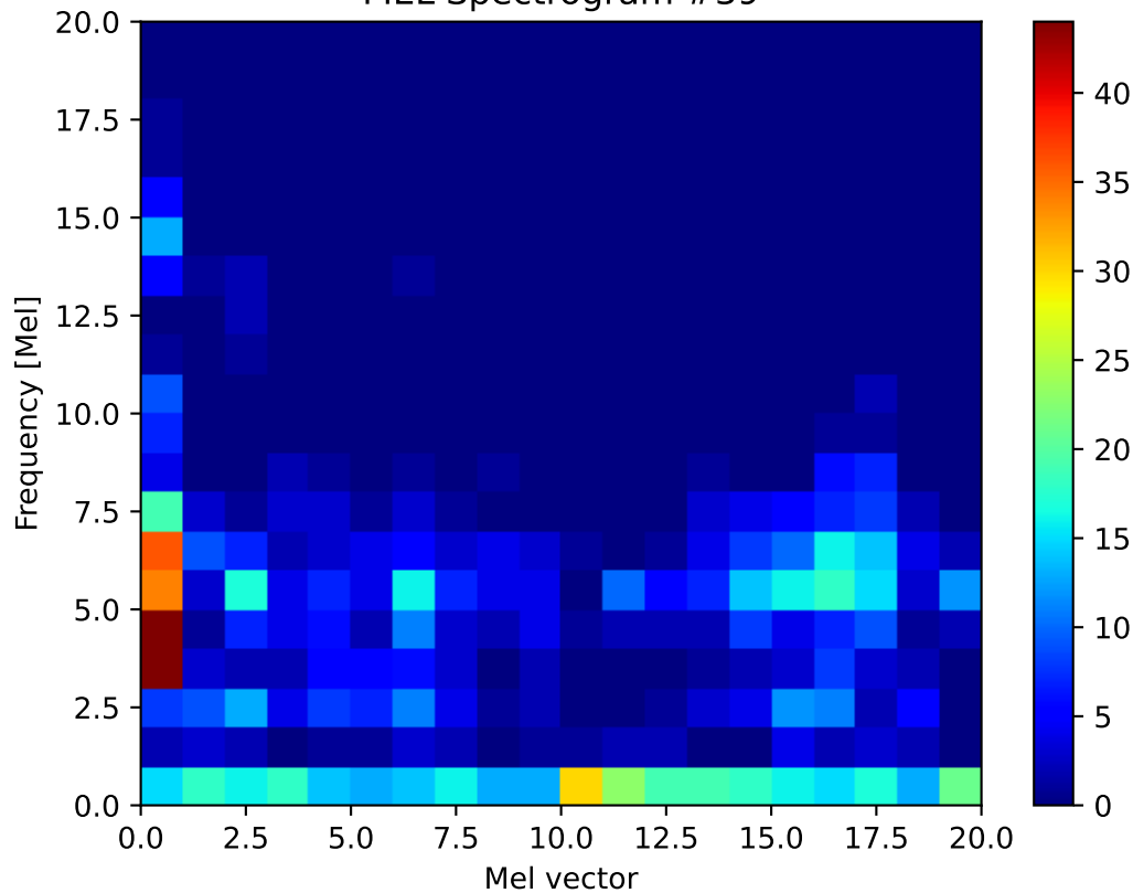
MEL Spectrogram #39
